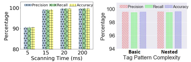
Figure 17: Tag identification with different scanning time.
